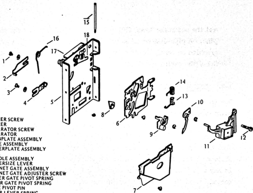
COIN ACCEPTOR - EXPLODED
