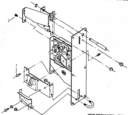
COIN MECHANISM - EXPLODED
