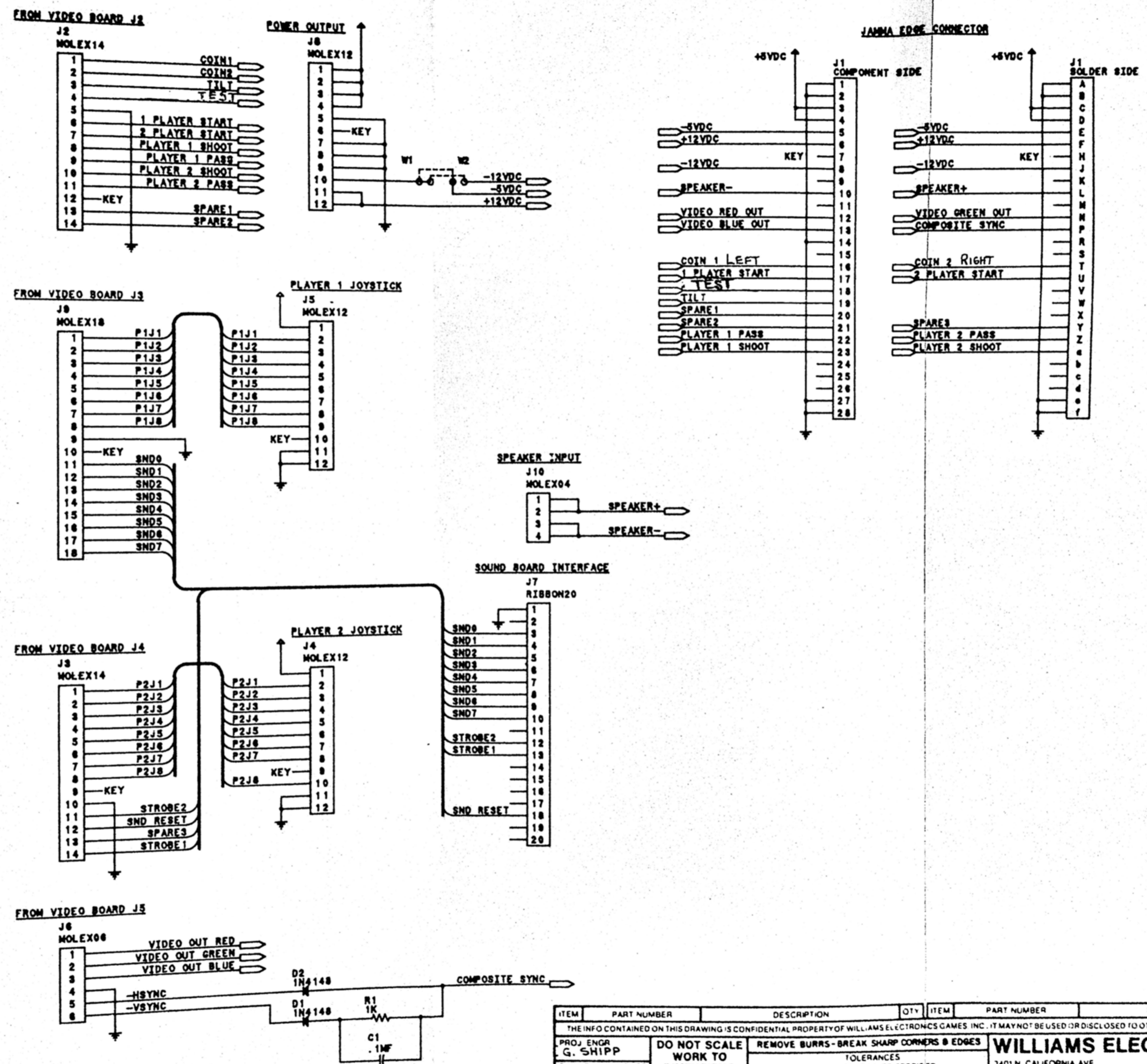
JAMMA INTERFACE BOARD SCHEMATIC
