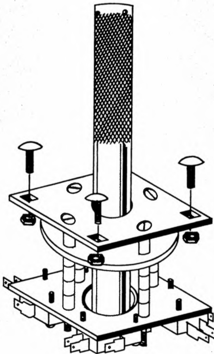
Figure 4, The Joystick Unit
