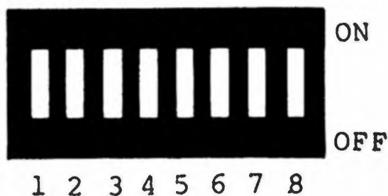
FIGURE 1, 8-Position DIP Switch
