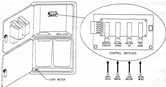
CONTROL SWITCH LOCATIONS
