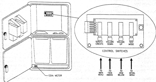
DIAGNOSTICS SUBMENU
