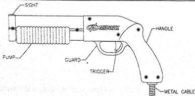
Shotgun Parts
