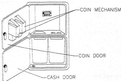
Interior View of Coin Door and Cash Door
