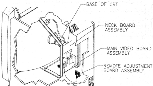
Cutaway Rear View
