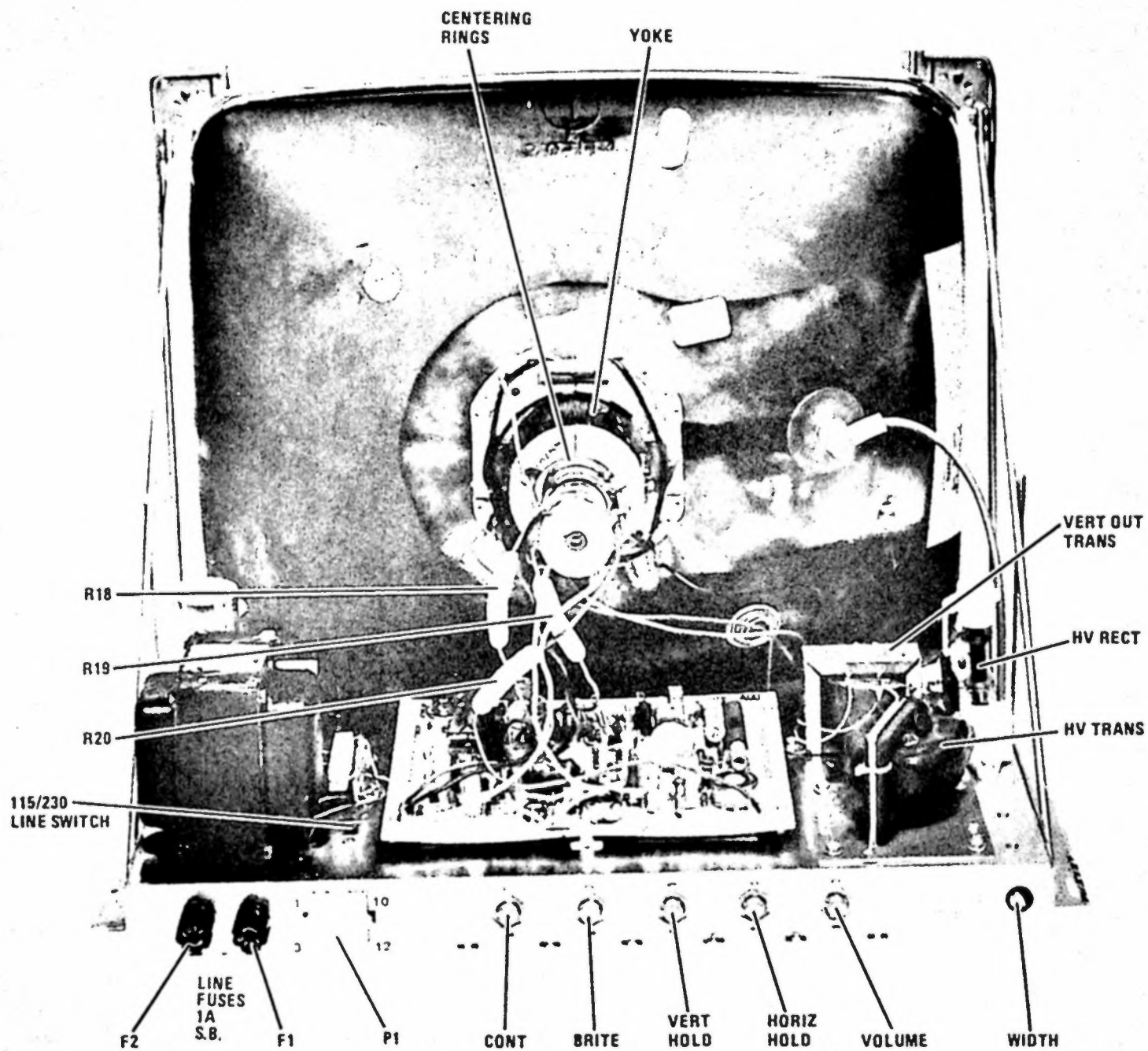
Chassis Component Location Rear View
