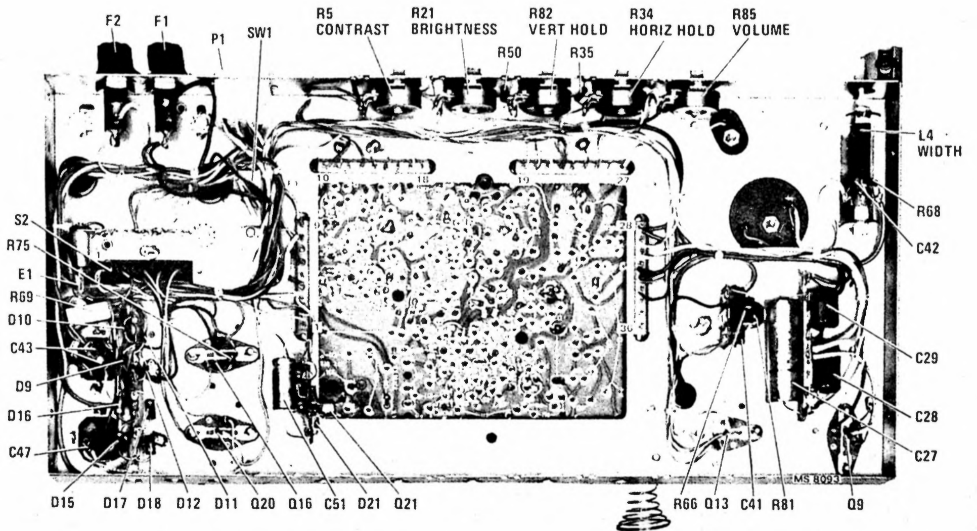
Chassis Component Location Bottom View
