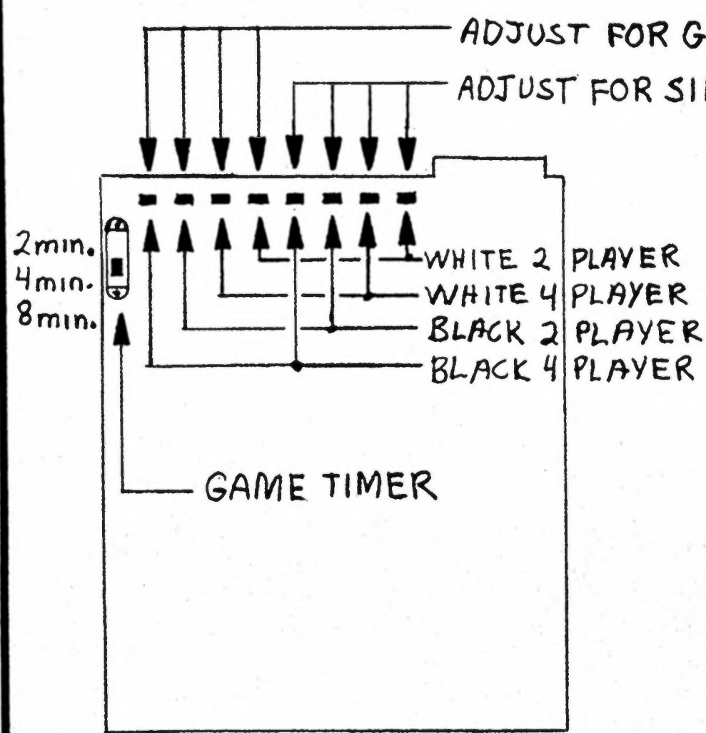
PCB FIGURE 3
