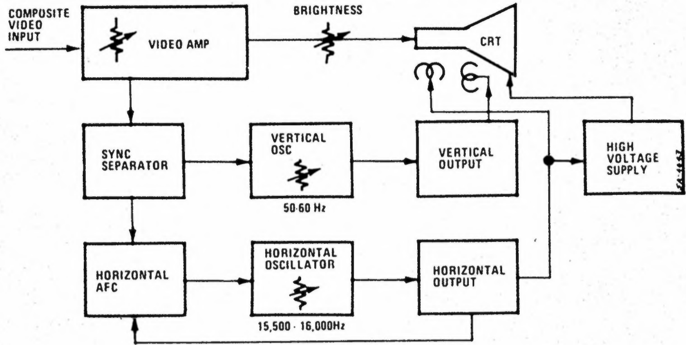
Block Diagram
