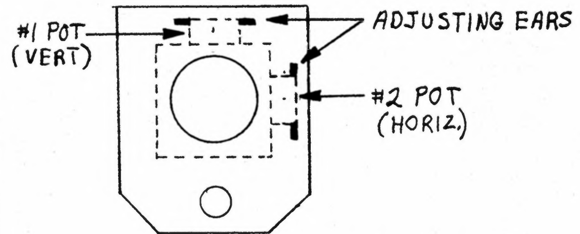
JOYSTICK W/ PLATE (TOP VIEW) FIGURE 1
