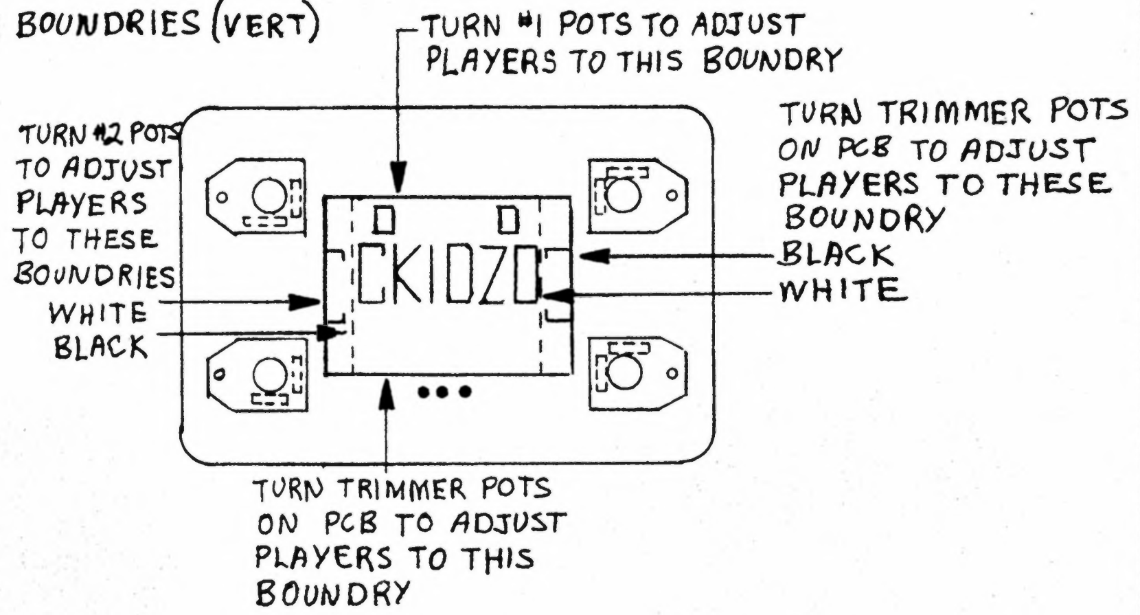
CABINET TOP (TOP VIEW) FIGURE 2
