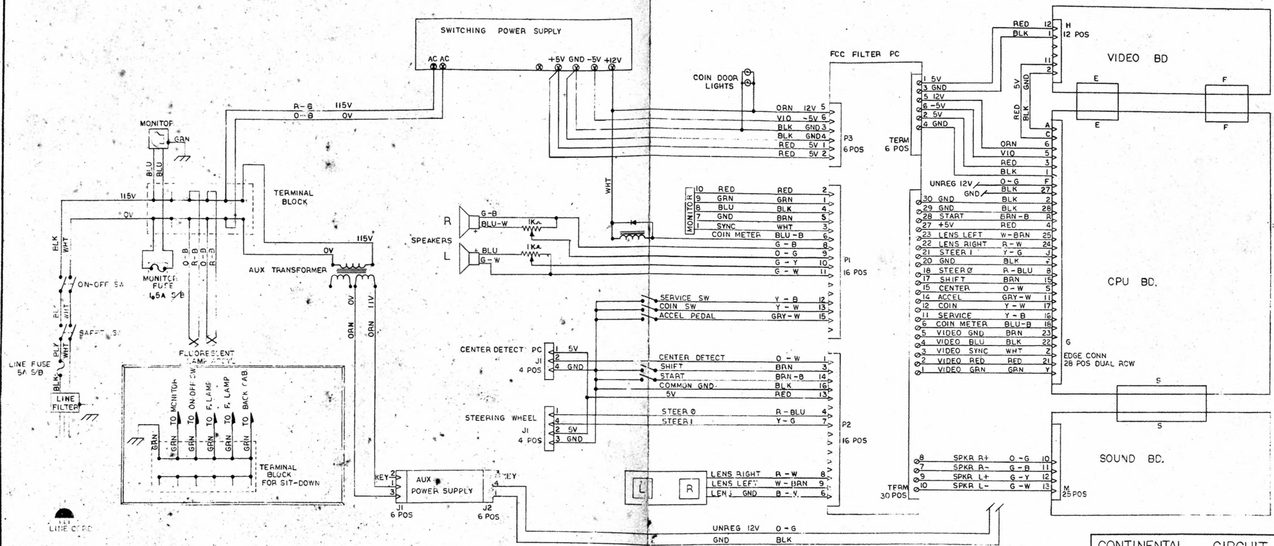
CONTINENTAL CIRCUIT SCALE: _____ APPROVED BY: _____ DRAWN BY: _____ DATE: _____ WIRING DIAGRAM TAITO _____ DRAWING NUMBER: _____
