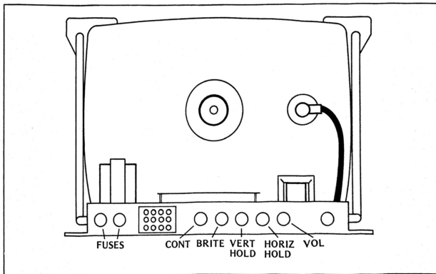
Figure 5-1 Location of Adjustments on TV Chassis
