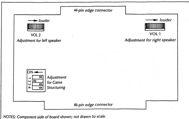
Figure 4-1 Adjustments on Audio and Switch Matrix PCB
