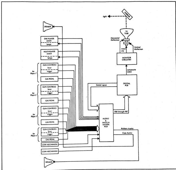
Figure 3-1 Functional Block Diagram of Cops 'N Robbers Game
