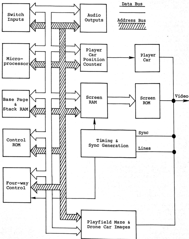
Figure 8: Logic Board Block Diagram
