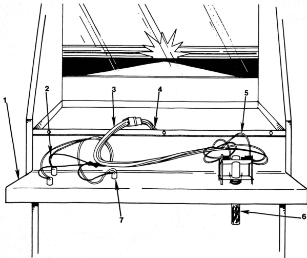
Figure 5: Control Panel (Late Production)
