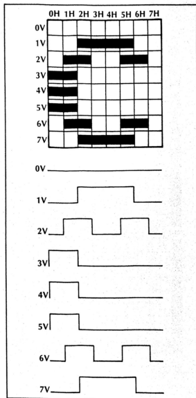
Figure 4-5 Playfield Generator Character Trace for the Letter "C"
