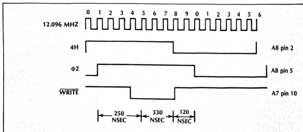
Figure 4-3 RAM Write Enable Signal Shaping
