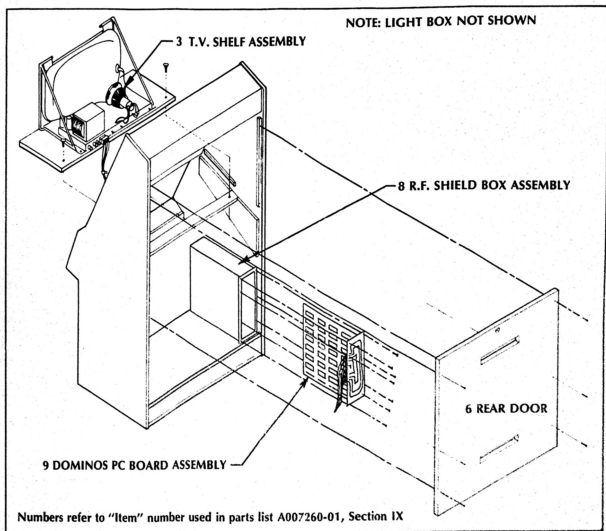
Figure 6-1A Exploded Diagram, Rear View
