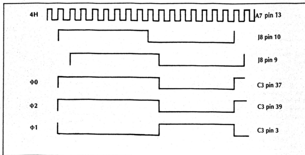
Figure 4-2 Phase 1 and Phase 2 Signal Shaping
