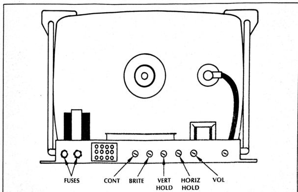
Figure 6-1 Location of Adjustments on TV Chassis
