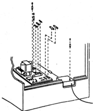
FUSE REPLACEMENT FIGURE 3
