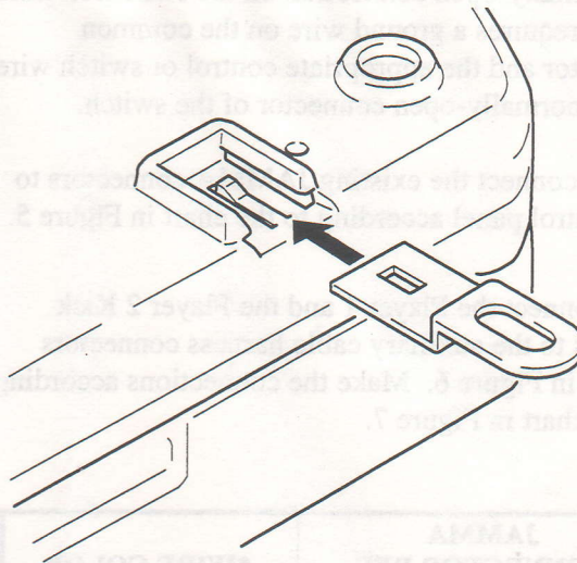
Figure 10: Mounting Bracket Installation
