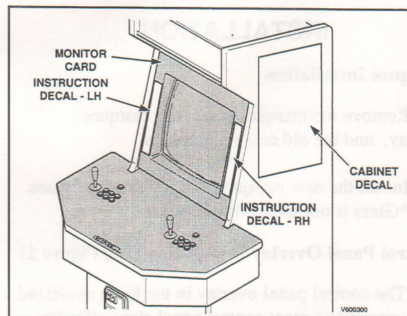
FIGURE 5 Cabinet Decal Installation
