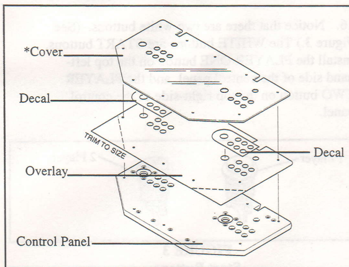
Figure 1 Overlay Installation
