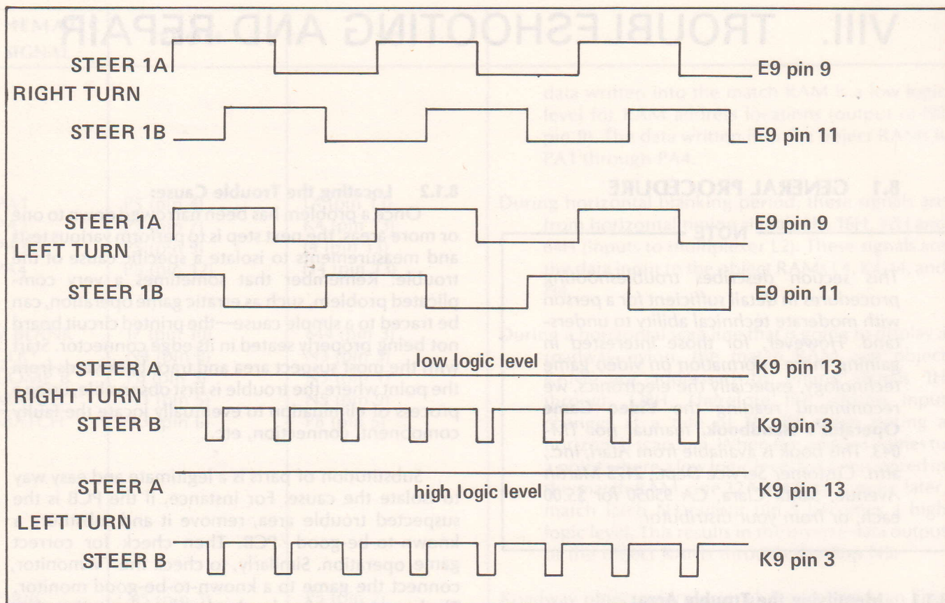
Figure 8-1 Steering Signals
