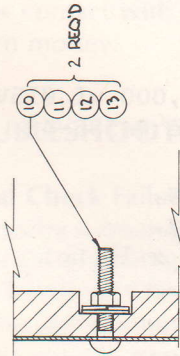
DETAIL - V
