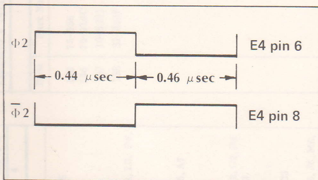
Figure 4-2 \Phi 2 and \overline{\Phi 2} Signals
