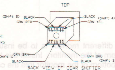
BACK VIEW OF GEAR SHIFTER
