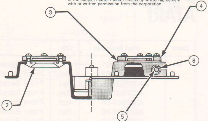
Figure 5-5 Front Bezel Assembly A007637-01 thru -07 D
