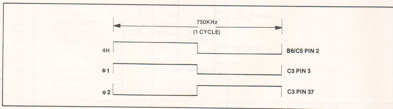
Figure 3-8 \Phi 1 and \Phi 2 Clock Driver Signal
