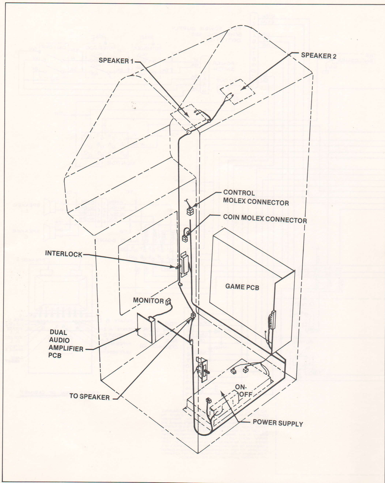
Figure 5 Orbit Game Harness Layout
