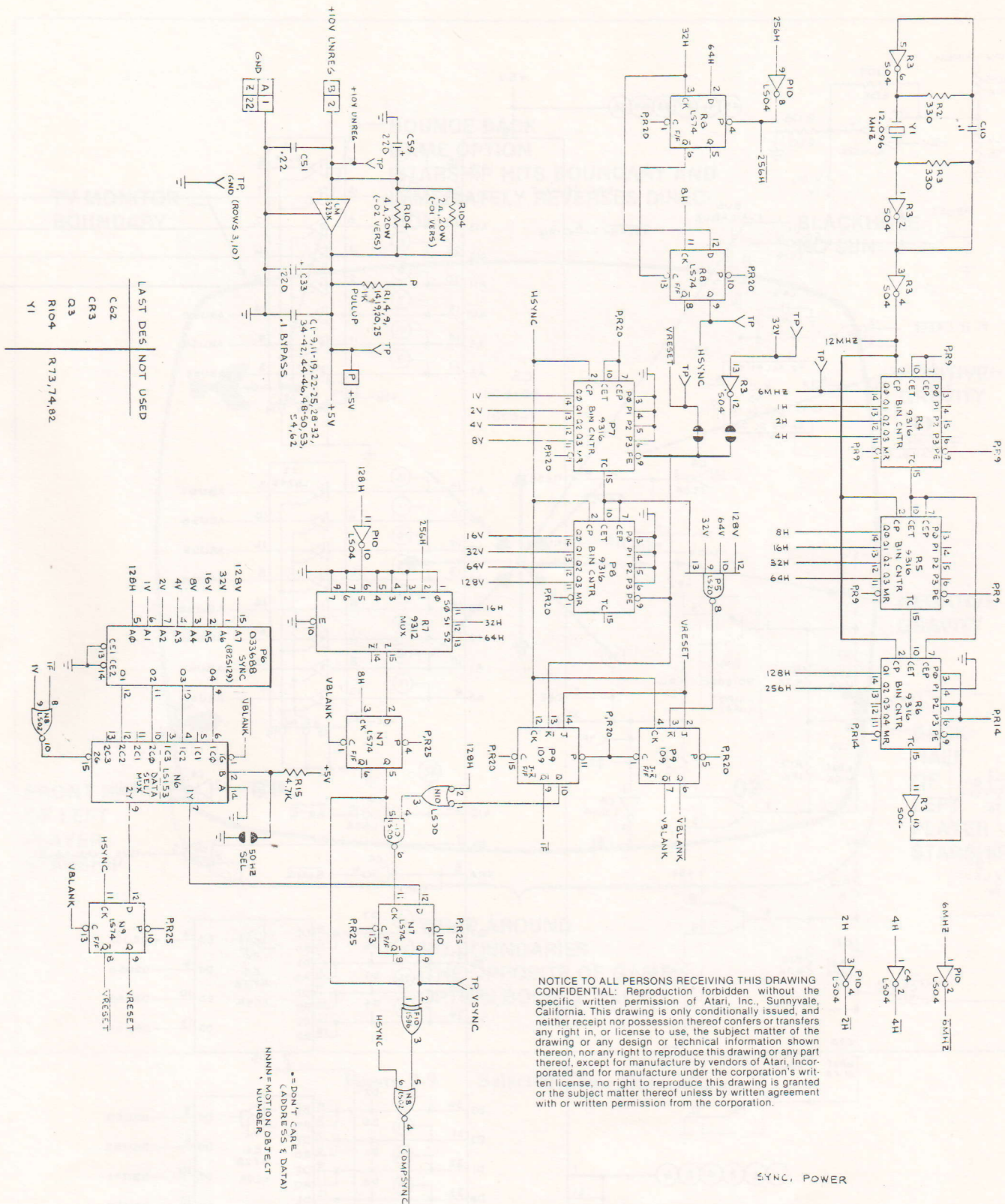
Figure 1 Orbit PCB Schematic Diagram Sheet 1 of 6 033570-01, 02
