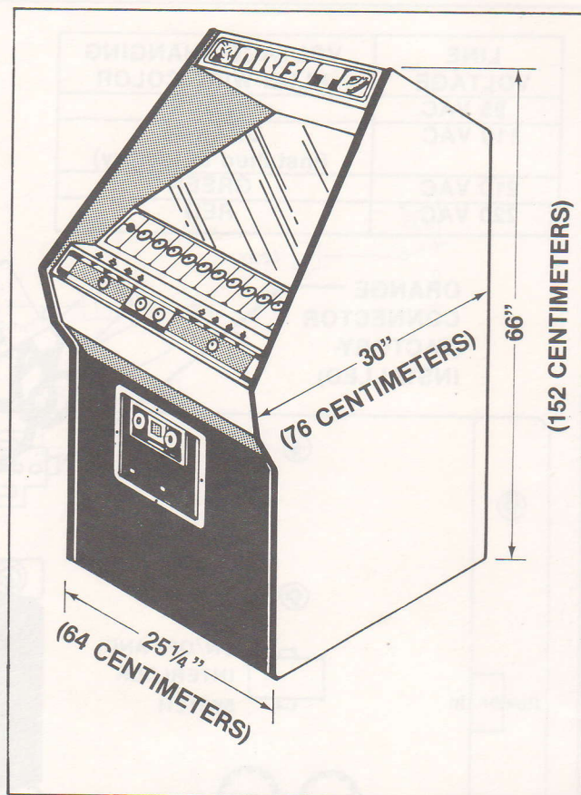
Figure 1-4 Location Set-up Requirements
