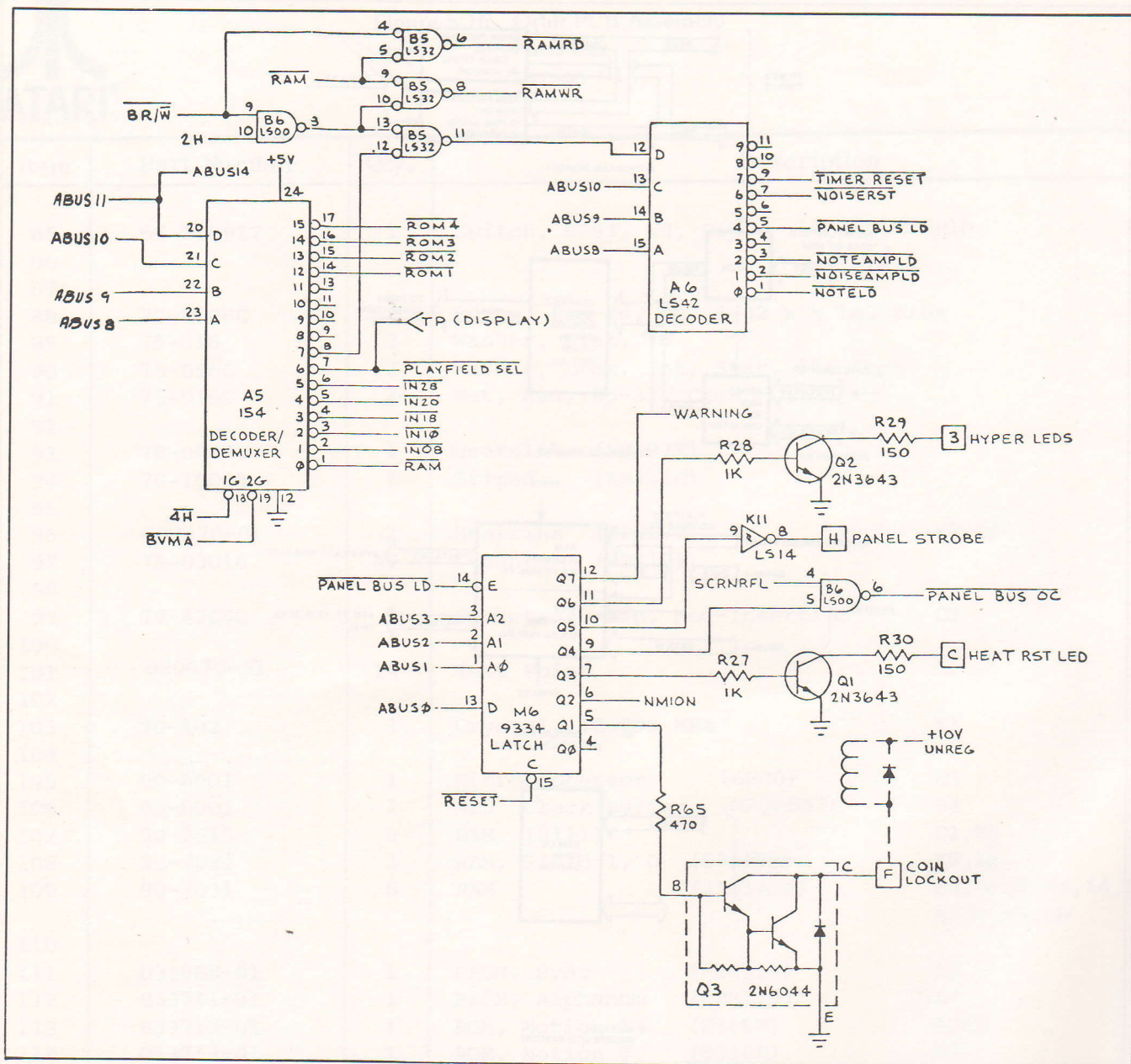
Figure 3-7 Address Decoding
