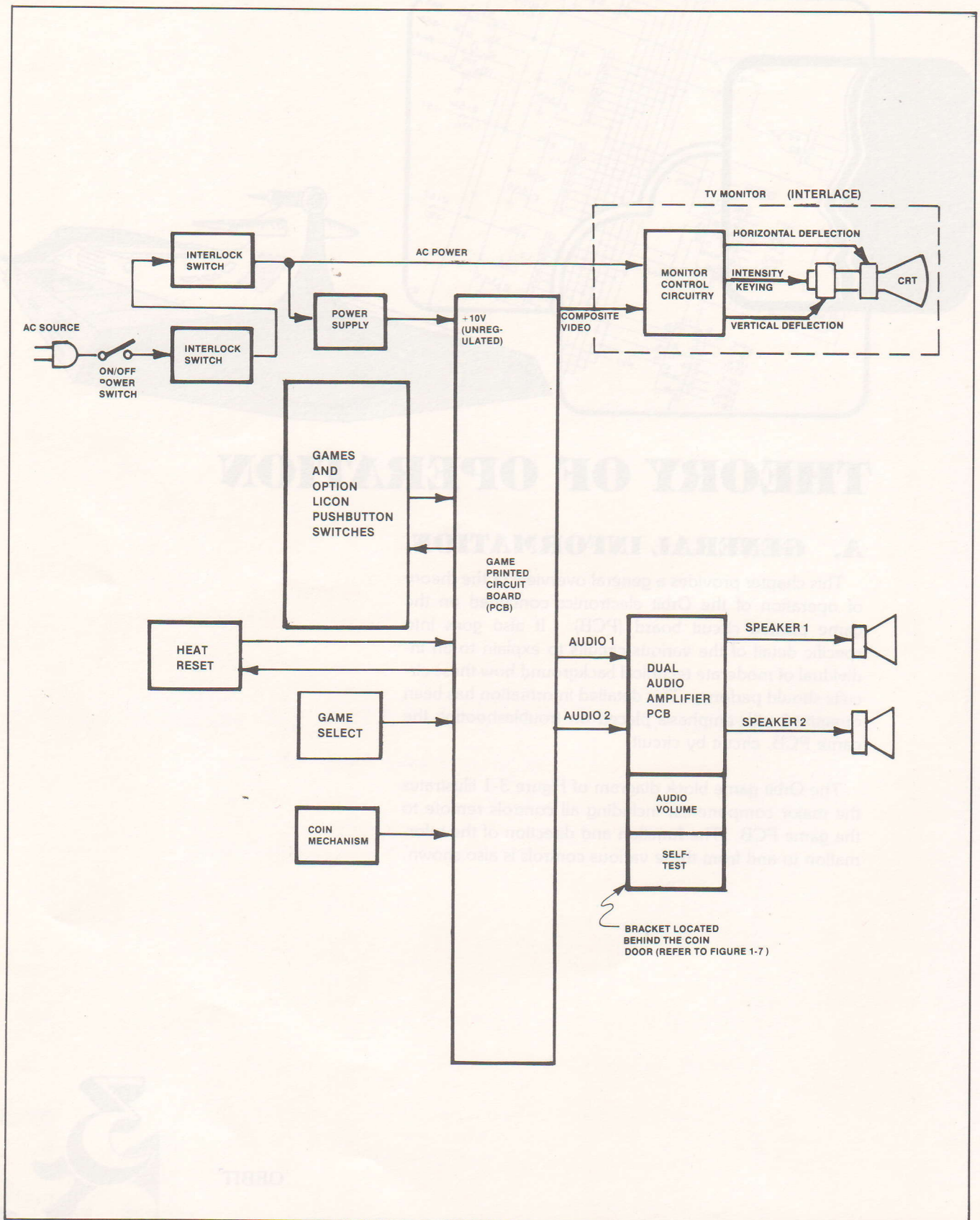
Figure 3-1 Orbit Game Block Diagram
