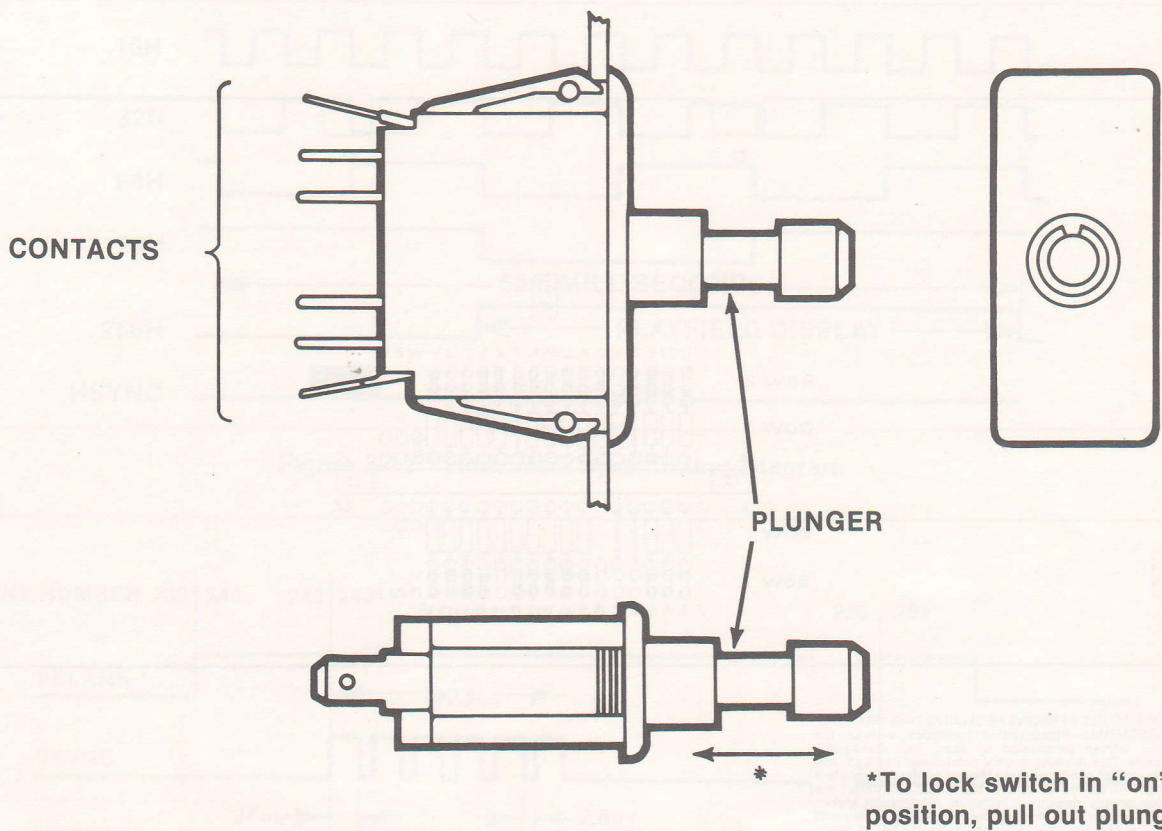
Figure 5-12 Interlock Switch Assembly 62-002
