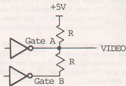
Figure 3-4 Simplified Video Circuit
