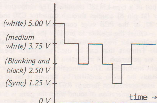
Figure 3-5 Waveform at Composite Video Point, (Junction of Resistors R15, R17, R18)
